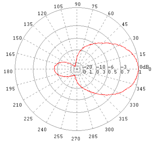
H-Ebene / H-Plane 0.8 GHz
