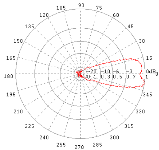
H-Ebene / H-Plane 7 GHz
