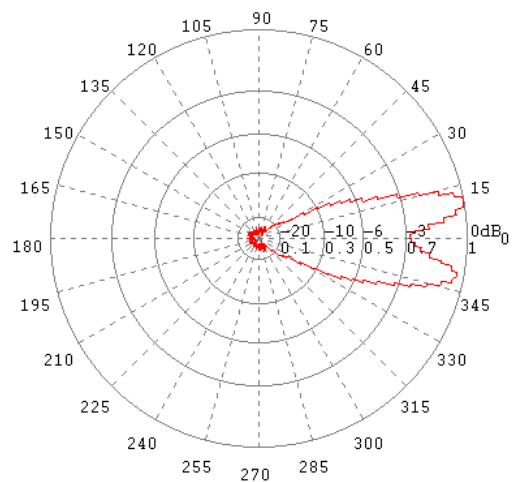
H-Ebene / H-Plane 8 GHz
