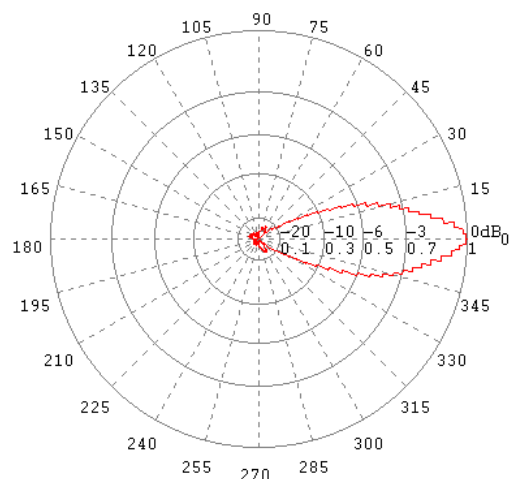
H-Ebene / H-Plane 6 GHz
