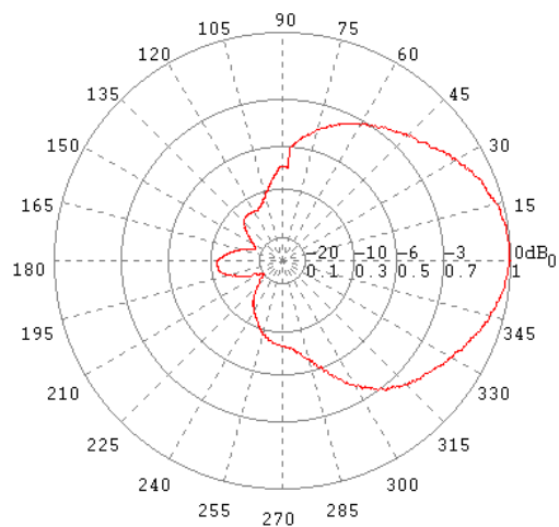
E-Ebene / E-Plane 1 GHz
