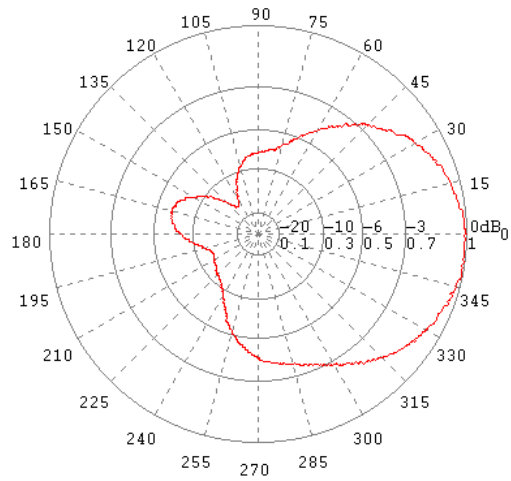
E-Ebene / E-Plane 0.8 GHz
