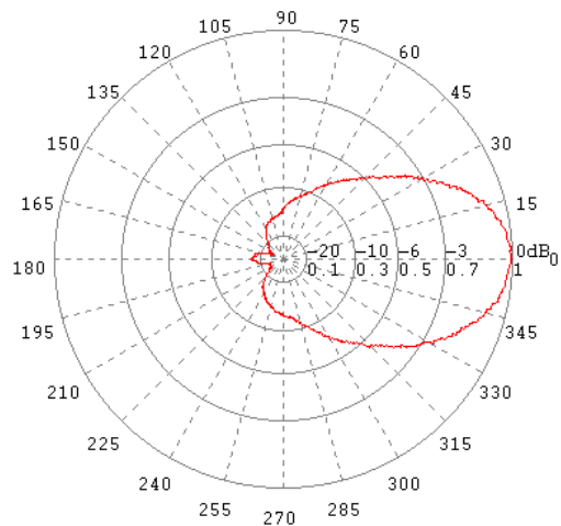
E-Ebene / E-Plane 1.5 GHz
