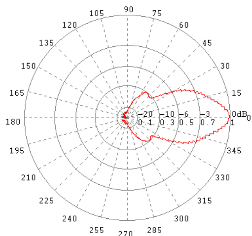
E-Ebene / E-Plane 6 GHz
