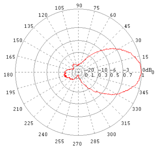
H-Ebene / H-Plane 1 GHz
