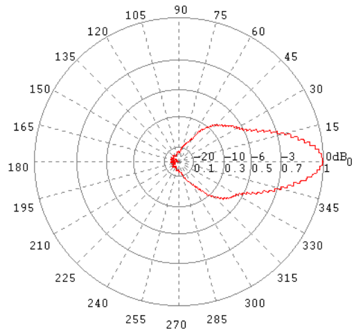
E-Ebene / E-Plane 4 GHz
