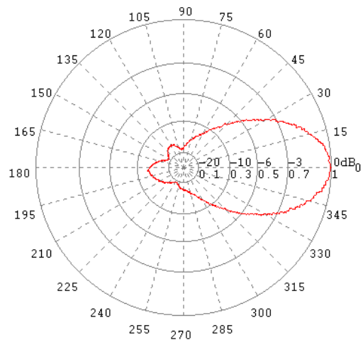
H-Ebene / H-Plane 1.5 GHz
