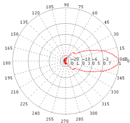
E-Ebene / E-Plane 9 GHz
