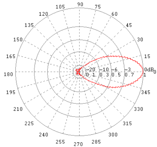
H-Ebene / H-Plane 4 GHz
