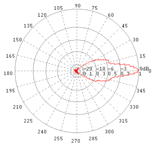
H-Ebene / H-Plane 9 GHz
