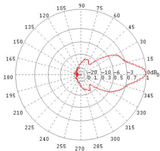
E-Ebene / E-Plane 5 GHz
