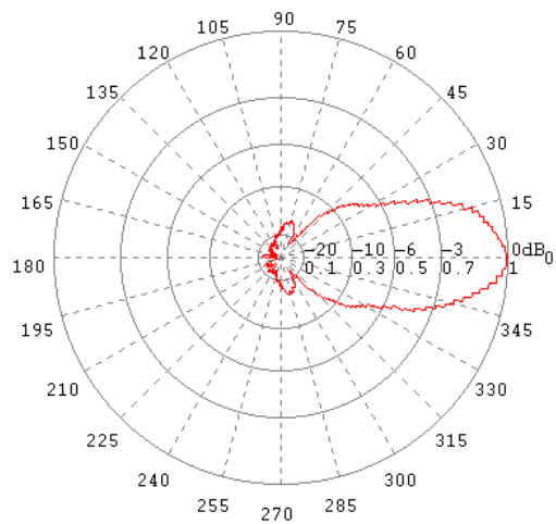
E-Ebene / E-Plane 7 GHz
