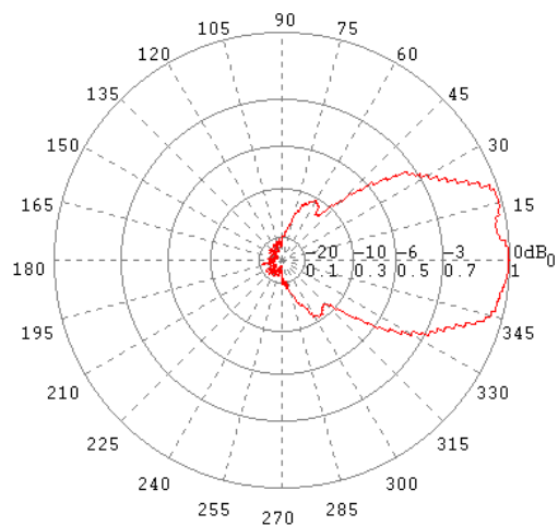
E-Ebene / E-Plane 8 GHz
