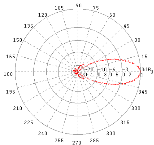
H-Ebene / H-Plane 5 GHz
